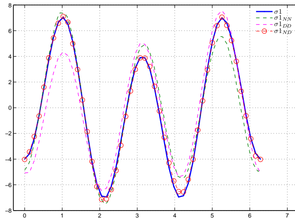
Figure 4. First test : The reconstructed stress on \Gamma_c
