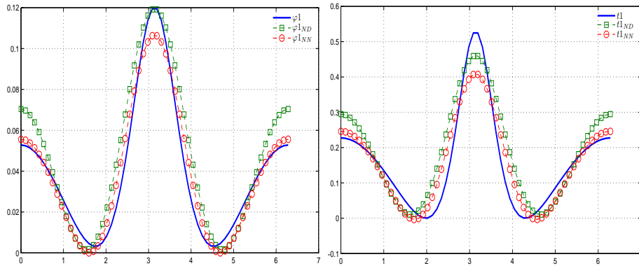
Figure 5. Singular data test : reconstructed velocity and the stress tensor on \Gamma_i
