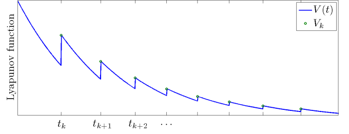
Fig. 2. Time evolution of Lyapunov function V .
