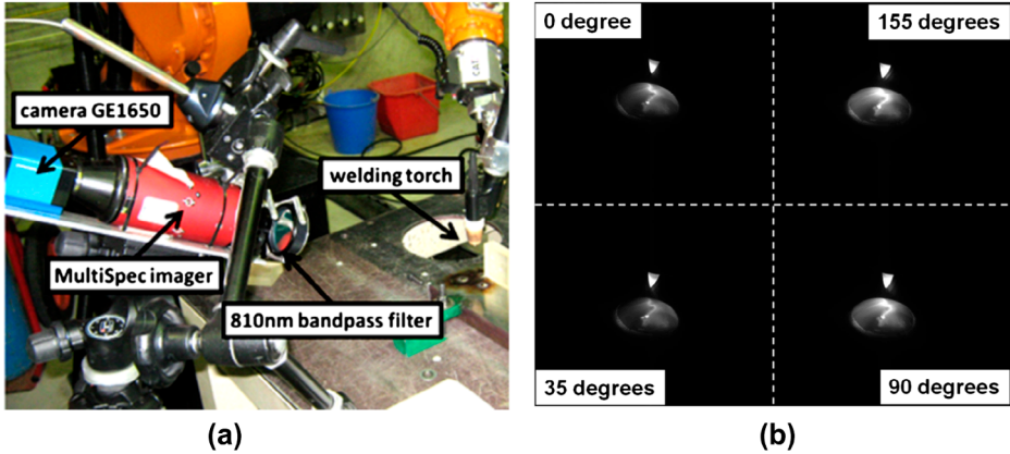
Figure 2. (a) Division of aperture polarimetric system, and (b) raw focal-plane image (1200 × 1600 pixels) showing four polarisation channels at indicated orientation.
