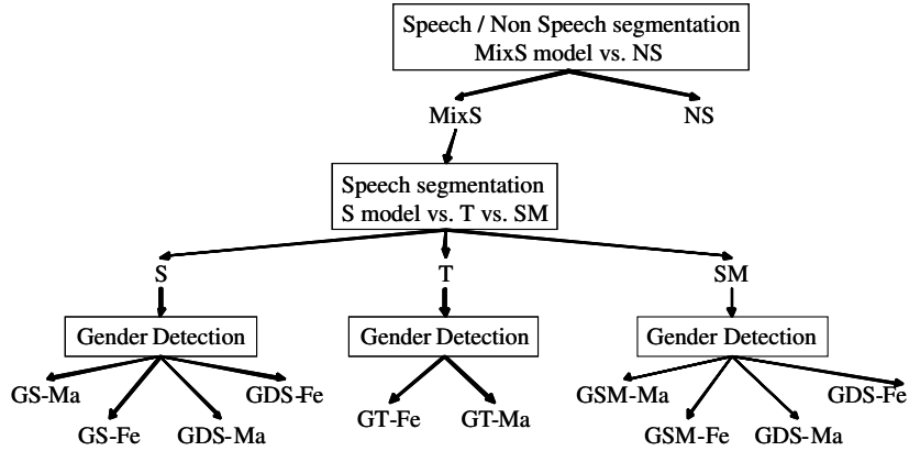
Fig. 2. Hierarchical acoustic segmentation
