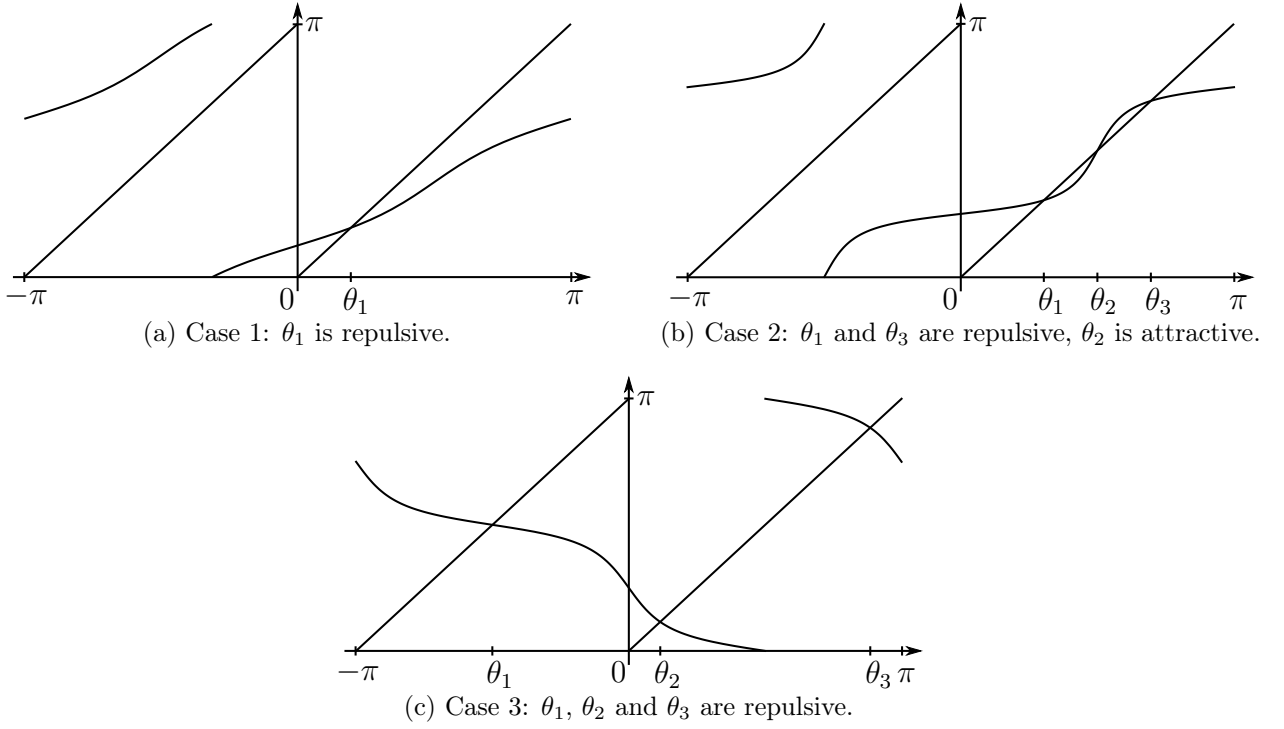
Figure 5: Examples of \phi_L in each of the three cases of Theorem 16. These specific examples correspond to L = \left( \begin{pmatrix} 3x \\ 2y \end{pmatrix}, \begin{pmatrix} 1 \\ 1 \end{pmatrix} \right) , L = \left( \begin{pmatrix} 4x \\ y \end{pmatrix}, \begin{pmatrix} 0 \\ 1 \end{pmatrix} \right) , and L = \left( \begin{pmatrix} x \\ -3y \end{pmatrix}, \begin{pmatrix} 0 \\ 1 \end{pmatrix} \right) respectively.
