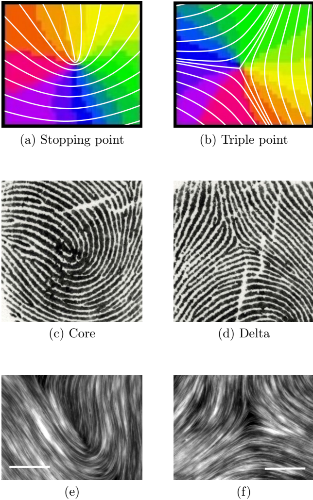
Figure 1: Examples of singularities observed in nature with half-integer indices.
