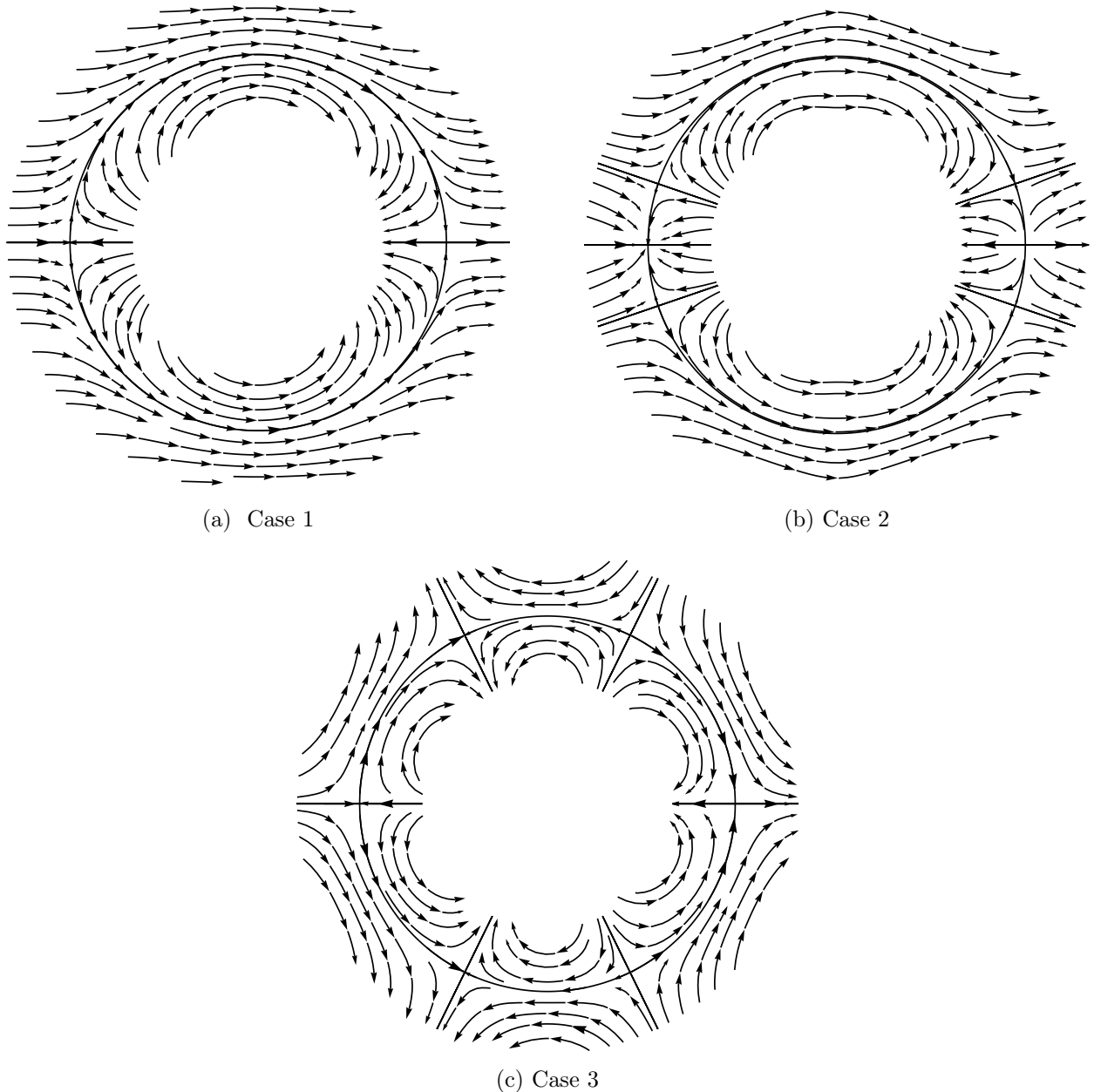
Figure 7: Examples of P in each case of Theorem 16, where (-\delta_0, \delta_0) \times (\mathbb{R}/4\pi\mathbb{Z}) is represented as an annulus. The figures 7a, 7b and 7c were respectively computed with Y = \begin{pmatrix} 1 \\ 0 \end{pmatrix} and X = \begin{pmatrix} x \\ 10y/11 \end{pmatrix} , X = \begin{pmatrix} x \\ 5y \end{pmatrix} , X = \begin{pmatrix} x \\ -3y \end{pmatrix} , respectively.
