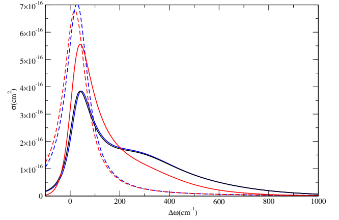
Fig. 9. Theoretical absorption cross sections of the components J_0 (blue line), J_1 (black line), and J_2 (red line) compared to the Lorentzian profiles for J_0 (blue/dash line) and for J_2 (red/dash line). The density of perturbers is n_{\text{He}} = 10^{21}\ \text{cm}^{-3} . The temperature is 6000 K.
