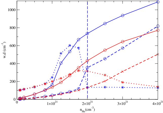
Fig. 12. Variation of the width (full line), shift (dashed line) and asymmetry \times 100 (dotted line) in the He density range n_{\text{He}} = 5 \times 10^{19} to 4 \times 10^{21} \text{ cm}^{-3} for T = 6000 \text{ K} . J_0 (blue lines) and J_2 (red lines).
