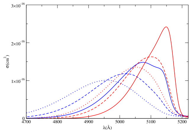
Fig. 11. Evolution of the unified profiles of the components J_0 (blue lines) and J_2 (red lines) with increasing helium density for n_{\text{He}} = 2 \times 10^{21} (full line), 3 \times 10^{21}\ \text{cm}^{-3} (dashed line) and 4 \times 10^{21}\ \text{cm}^{-3} (dotted line), T = 6000 K.
