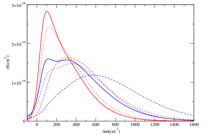
Fig. 10. Evolution of the unified profiles of the components J_0 (blue lines) and J_2 (red lines) with increasing helium density for n_{\text{He}} = 1.75 \times 10^{21} (full line), 2 \times 10^{21} (dotted line) and 3 \times 10^{21}\ \text{cm}^{-3} (dashed line), T = 6000 K.
