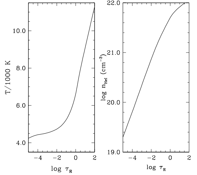
Fig. 6. Temperature and He density as a function of Rosseland mean optical depth assuming SDSS 1535+1247 atmospheric parameters (Koester et al. 2011).
