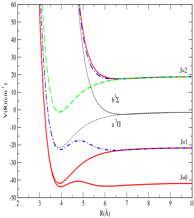
Fig. 2. Potential curves correlated with the 3p states without (black) and with inclusion of spin-orbit coupling (red/full: \Omega = 0 , blue/dash-dot: \Omega = 1 and green/dash: \Omega = 2 ) of the Mg–He molecule. The energies are given relative to the potentials without spin-orbit coupling. The fine structure separation is 20.2573 \text{ cm}^{-1} .
