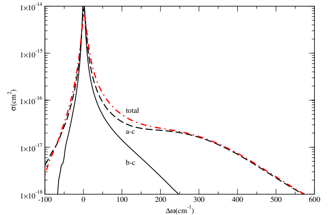
Fig. 4. Individual components of the line profile, neglecting the SO coupling, compared to the total profile at T = 6000 \text{ K} and for n_{\text{He}} = 10^{20} \text{ cm}^{-3} .
