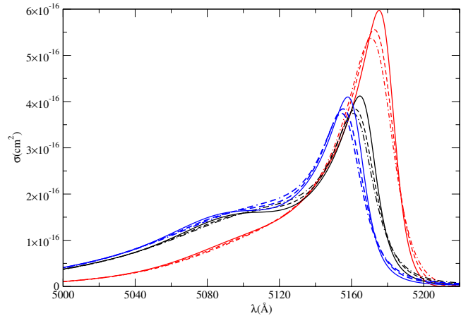
Fig. 7. Variation of the line profile with temperature for n_{\text{He}} = 10^{21} \text{ cm}^{-3} for the 3 components J_0 (blue line), J_1 (black line), and J_2 (red line). 4000 K (full line), 6000 K (dashed line), and 8000 K (dashed dotted line).
