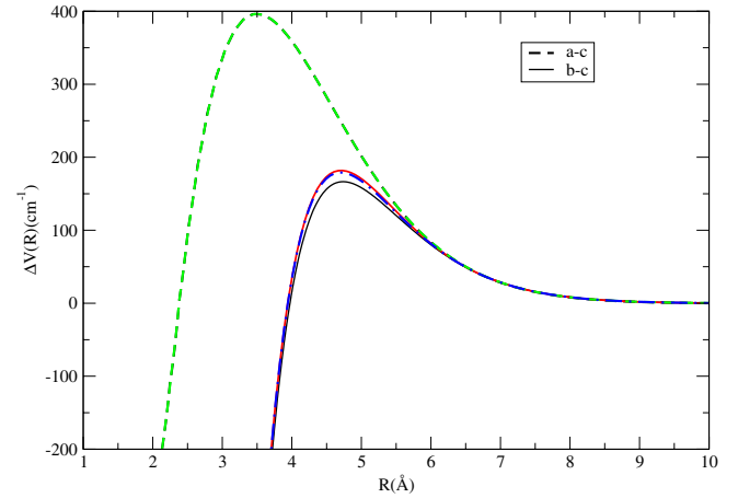
Fig. 3. \Delta V for the transitions contributing to 3p \rightarrow 4s line without SO (black lines): 3p^3\Sigma \rightarrow 4s^3\Sigma and 3p^3\Pi \rightarrow 4s^3\Sigma . All the other \Delta V for the components J = 2 are superimposed (red/full: \Omega = 0 , blue/dash-dot: \Omega = 1 and green/dash: \Omega = 2 ).
