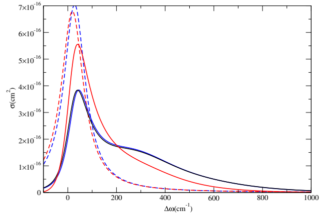
Fig. 9. Theoretical absorption cross sections of the components J_0 (blue line), J_1 (black line), and J_2 (red line) compared to the Lorentzian profiles for J_0 (blue/dash line) and for J_2 (red/dash line). The density of perturbers is n_{\text{He}} = 10^{21}\ \text{cm}^{-3} . The temperature is 6000 K.
