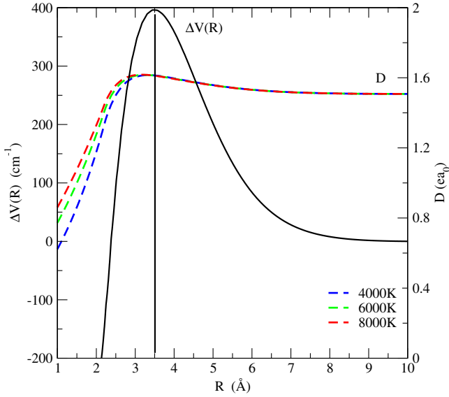
Fig. 8. Difference potential energy \Delta V(R) in \text{cm}^{-1} (black line) and the temperature dependence of modulated dipole D(R) (color lines) corresponding to the 3p\ a \rightarrow 4s\ c transition.
