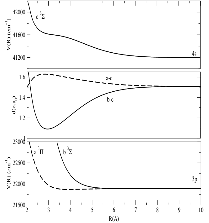
Fig. 1. Potential energies for the a , b , and c states of the Mg–He molecule without SO coupling. 4s c\ ^3\Sigma (full line), 3p b\ ^3\Sigma (full line), 3p a\ ^3\Pi (dashed line), and transition dipole moment c - b (full line), c - a (dashed line).
