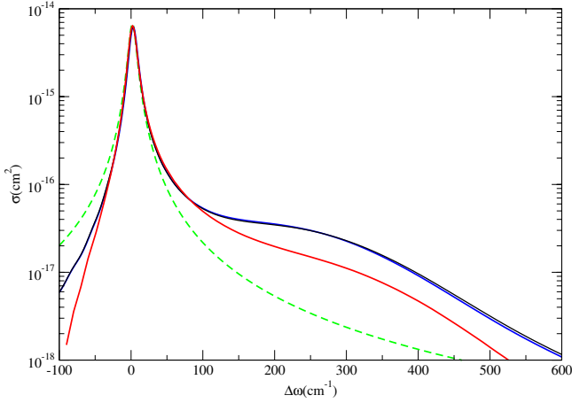
Fig. 5. Theoretical absorption cross sections of the components J_0 (blue line), J_1 (black line), and J_2 (red line) compared to the Lorentzian profile for J_2 (green/dash line). The density of perturbers is n_{\text{He}} = 10^{20} \text{ cm}^{-3} . The temperature is 6000 K.
