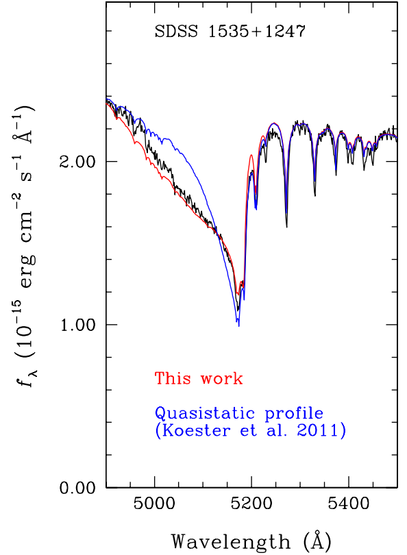
Fig. 13. Comparison of the Mg line profiles using the quasistatic profile (blue) and the unified line-shape semi-classical theory (red) for SDSS 1535+1247 (black line). The atmospheric parameters of Koester et al. (2011) are assumed.
