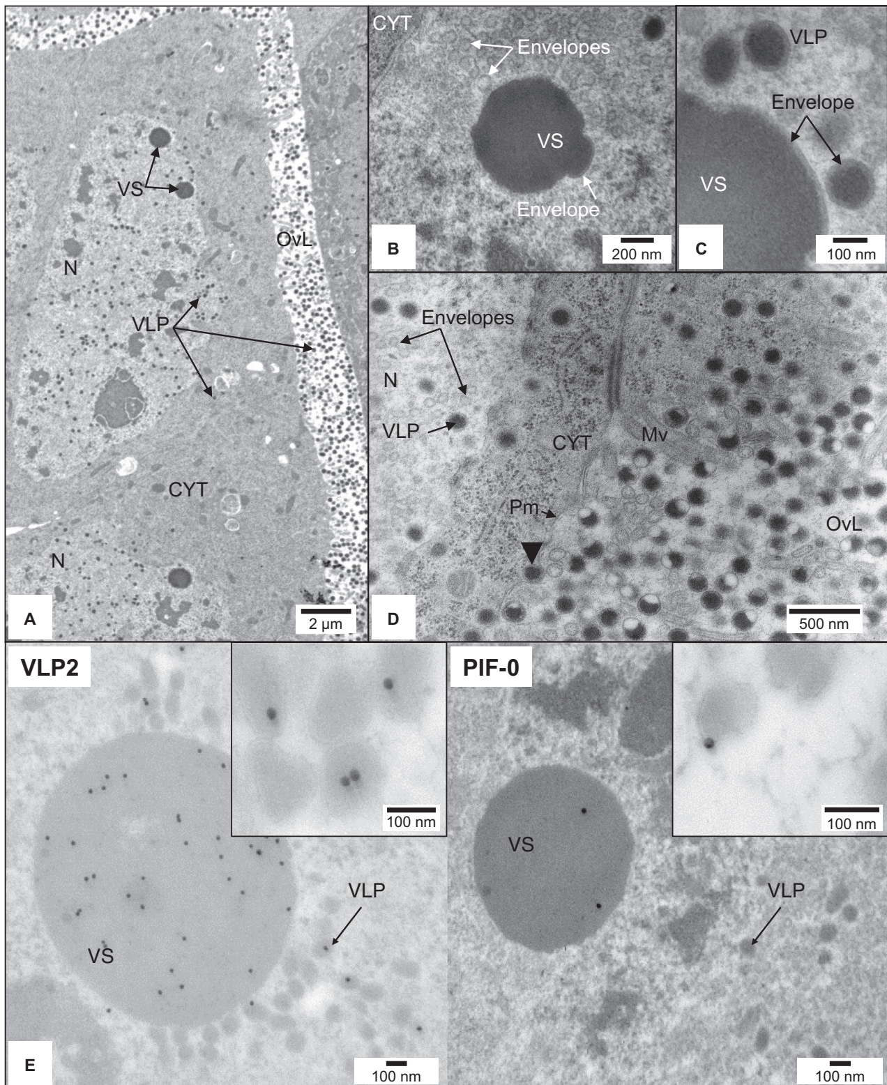
Fig. 1. VLP morphogenesis in V. canescens calyx cells. (A to E) Transmission electron micrographs of (A) calyx cells displaying hypertrophic nuclei (N) containing virogenic stroma (VS) and VLPs; (B) calyx cell nuclei with empty envelopes close to the VS; (C) envelopes filled with VS material giving rise to VLPs; (D) VLPs budding from the calyx cell membrane; (E) immunogold labeling of VS and VLPs in the nucleus with specific antibodies against VLP2 ( left ) and PIF-0 ( right ). ( Insets ) Larger magnifications of VLPs. CYT, cytoplasm; Mv, microvilli of the cytoplasmic membrane; OvL, oviduct lumen; Pm, plasma membrane.
