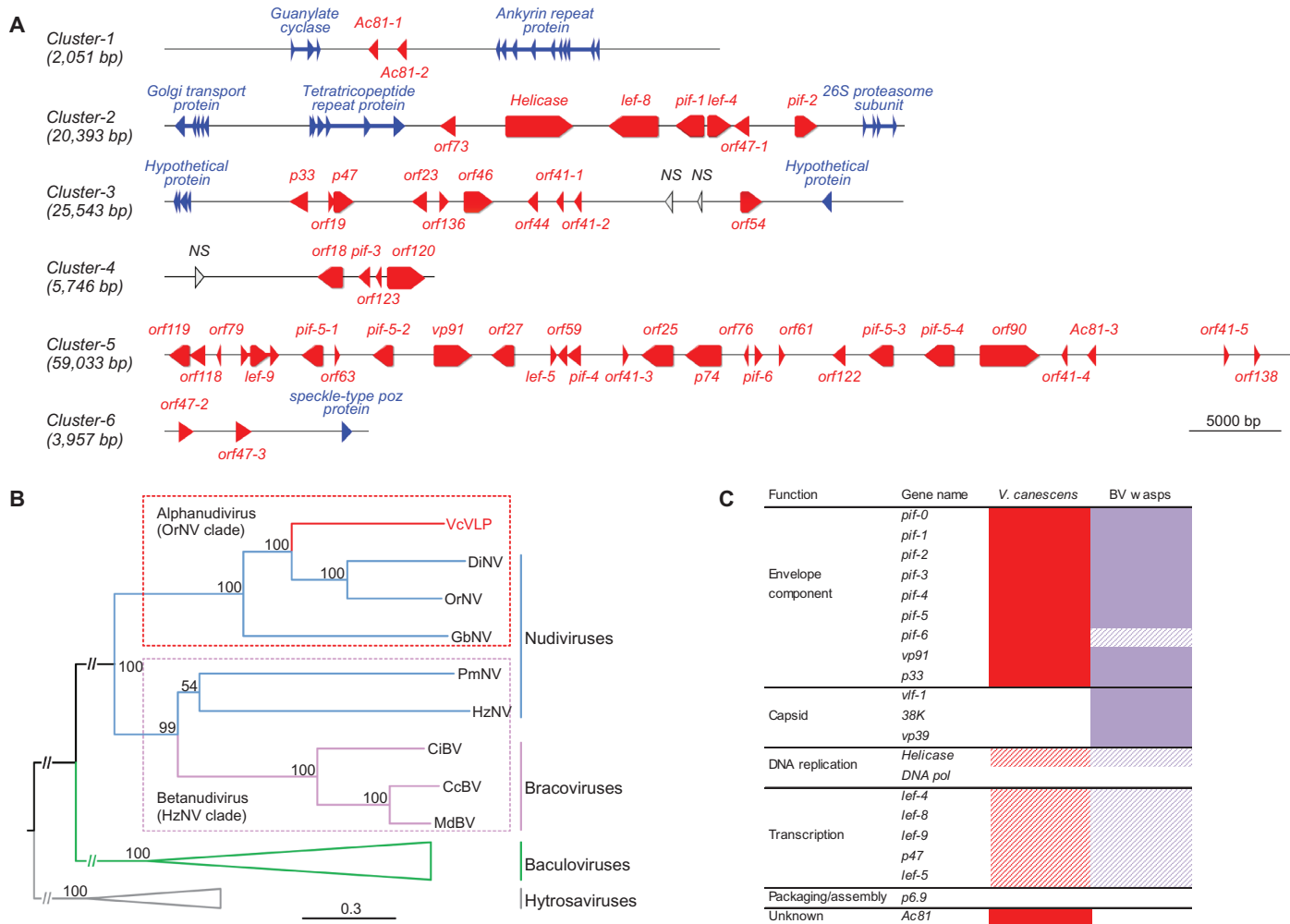
Fig. 2. Organization, origin, and putative function of the nudiviral genes of the V. canescens genome. (A) Nudiviral genes (in red; named after their OrNV homologs) are grouped into six clusters flanked by regions containing conserved wasp genes (in blue). (B) Phylogenetic tree of insect large double-stranded DNA viruses obtained by maximum likelihood analysis with a concatenated multiple alignment for 37 genes showing that the nudiviruses captured by the V. canescens and braconid wasp lineages belonged to different clades. VcVLP, V. canescens VLP. (C) Genes common to nudiviruses and baculoviruses conserved in V. canescens (red) or wasps carrying bracoviruses (BV) (purple). The products of the helicase gene and of the genes mediating viral gene transcription are not incorporated into the particles (hatched motif). Note that V. canescens lacks capsid genes, consistent with the absence of DNA in the particles.
