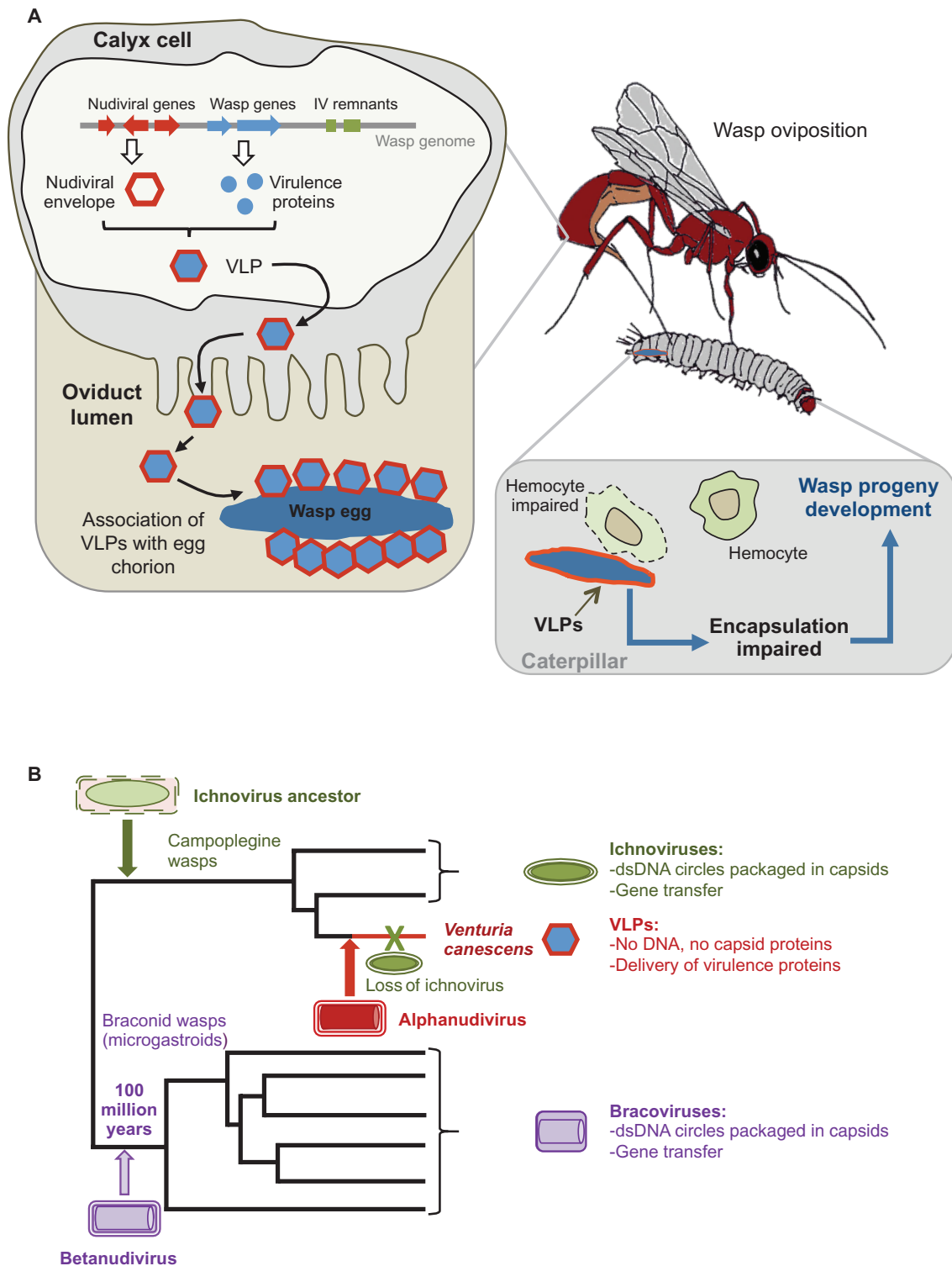
Fig. 3. Overview of the production, function, and origin of V. canescens VLPs. (A) VLPs consist of virulence proteins of wasp origin wrapped in nudiviral envelopes. VLPs are released into the oviduct lumen, where they become attached to the wasp egg. Once in the parasitized caterpillar host, VLPs confer immune protection to the egg by impairing capsule formation by the host immune cells. (B) Recurrent virus domestication during parasitic wasp evolution. Two virus genome integration events have occurred during the evolution of campoplegine wasps: the first involved a genome, making it possible to produce ichnoviruses (mediating gene transfer), and the second involved an alphanucleovirus genome used for VLP production (mediating the delivery of virulence proteins), which has replaced the ichnovirus in V. canescens . A betanucleovirus was independently acquired by a braconid wasp ancestor and gave rise to bracoviruses (DNA delivery).
