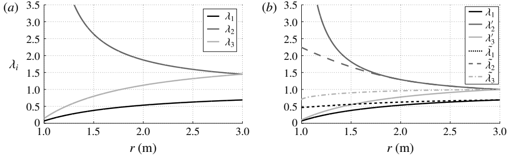
FIGURE 2. (a) Parameters \lambda_i of the geometric transformation for a = 1 m, b = 3 m, r_0 = 0.1 m. (b) Parameters \lambda'_i defined to adapt the seabed at r = b and parameters \tilde{\lambda}_i .
