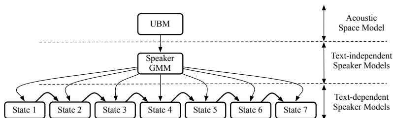
Figure 1: General view of the EBD architecture.
