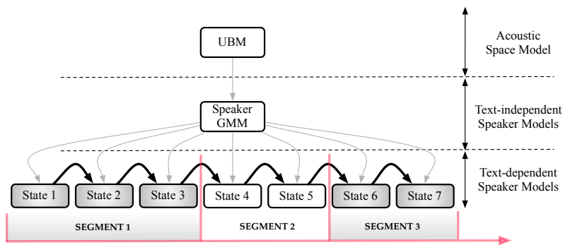
Figure 2: General view of the EBD architecture integrating additional TSI in the form of three overarching segments.
