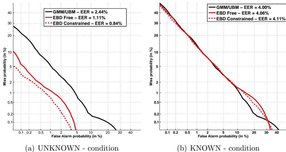
Figure 5: Detection Error Trade-off curves of the GMM-UBM baseline and EBD system with 20 states per SCHMM, with free or constrained Viterbi alignment. Cases where the imposters do not know the client pass-phrase and pronounce a different utterance (UNKNOWN - condition) and where the imposters know the client pass-phrases (KNOWN - condition)
