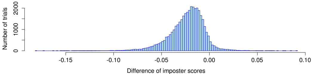
Figure 7: Distribution of imposter score differences, between Viterbi decoding with and without lexical constraint, when imposters do not know the client pass-phrase and pronounce a different utterance (UNKNOWN).
