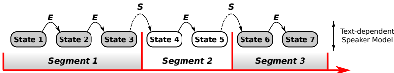
Figure 3: Use of a lexical synchronization in the bottom layer of the EBD architecture constrains the Viterbi decoding and increases the discriminative power of the system. In this example, the synchronization signal consists of 2 discrete points separating 3 overarching segments. Transitions E are fixed and set to equiprobability while transitions S value varies during the decoding.
