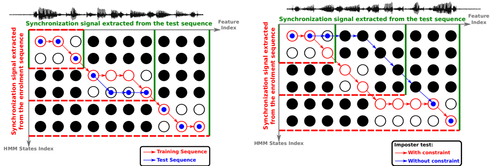
(a) Viterbi alignment of client training and test utterances with a lexical constraint applied during the decoding. (b) Alignment of imposter utterance with and without lexical constraint.
