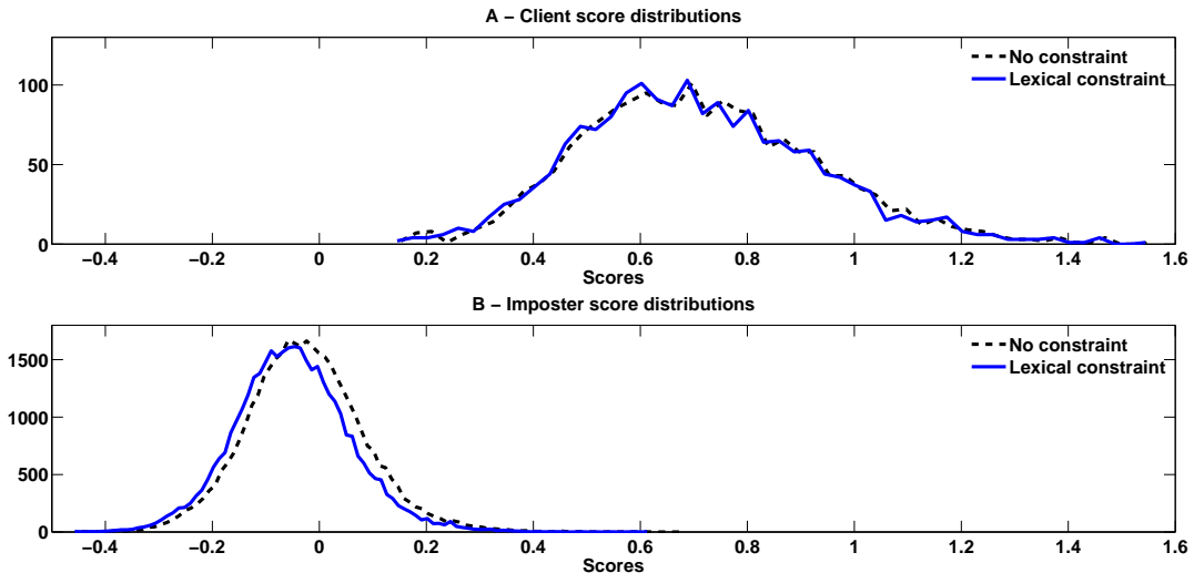
Figure 6: Evolution of the client and imposter text-dependent score distributions when using additional information coming from a lexical synchronization (constrained Viterbi decoding) or no synchronization information (classical Viterbi decoding). Case where imposters do not know the client pass-phrase and pronounce a different utterance (UNKNOWN).
