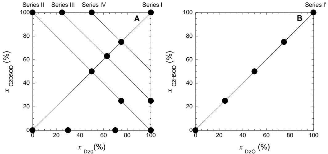
Figure 2. Water/ethanol (v/v 50/50) composition of the gluten gels studied by neutron scattering. (A) D6 group: samples prepared with a mixture of H_2O/D_2O/C_2H_5OH/C_2D_5OD (B) OD group: samples prepared with a mixture of H_2O/D_2O/C_2H_5OH/C_2H_5OD .
