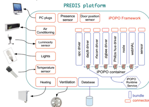
Figure 10: Sensor/actuators interoperability framework.
