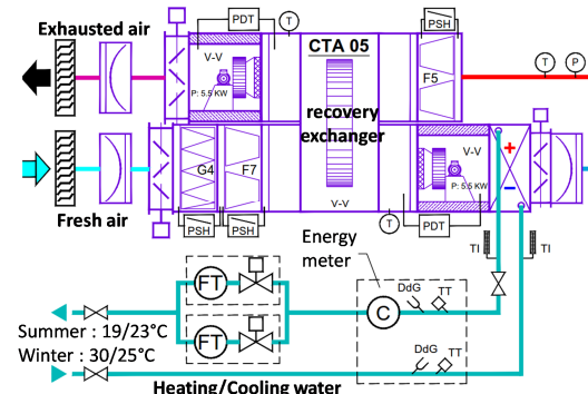
Figure 7: HVAC system.
