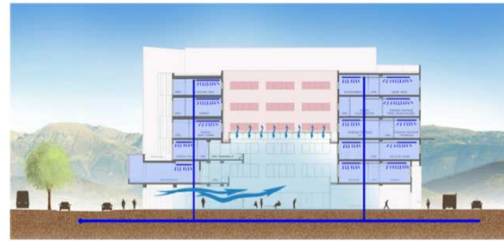
Figure 6: Natural ventilation through the atrium.
