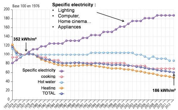
Figure 2: Evolution tendency of residential energy consumption /m² in France.
