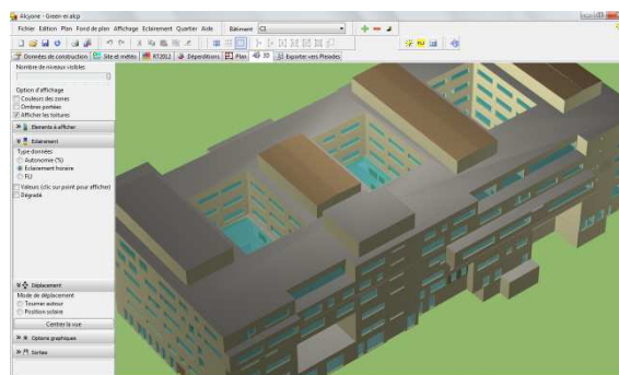
Figure 12: Thermal dynamic simulation of GreEn-ER (COMFIE software).
