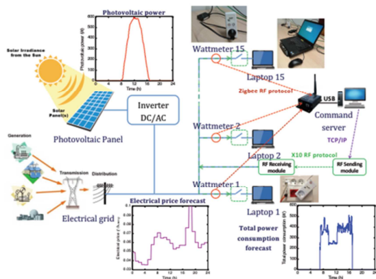
Figure 11: Real time control of 15 laptops charging/discharging for demand response.
