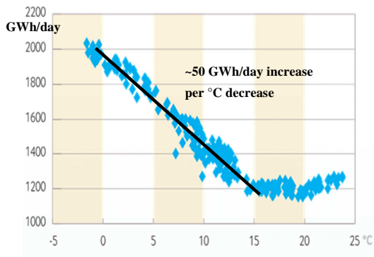
Figure 1: Correlation between temperature and electrical consumption in France – Gradient of daily consumption in France in GWh/day as a function of the average temperature in France (in °C).
