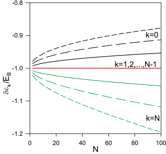
FIG. 4. Size dependence of the energy shifts \delta\epsilon_k for C = 0.01 and for B = 0.01 (full lines), B = 0.02 (long dashed lines), and B = 0.03 (short dashed lines).
