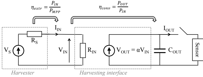
Fig. 1. Harvester electrical model and harvesting interface schematic.
