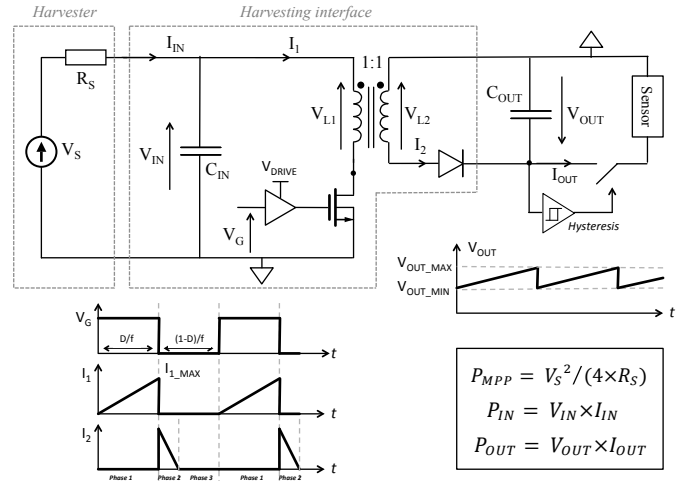
Fig. 2. Flyback converter working in DCM as harvesting interface.
