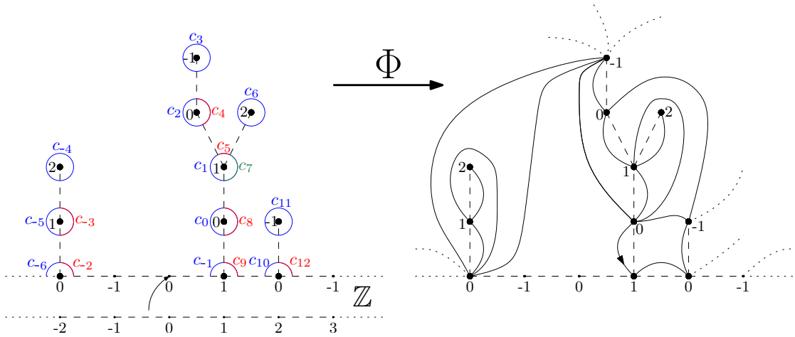
Figure 2: The Bouttier-Di Francesco-Guitter mapping. Vertex 0 of \mathbb{Z} is indicated by an arrow. The visible trees are attached to the vertices -2, 1 and 2 of \mathbb{Z} , which are labeled 0, 1 and 0, respectively. These vertices correspond to down-steps of the bridge.
