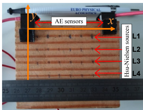
Figure 2: Wood specimen – AE sensors – Pencil lead
