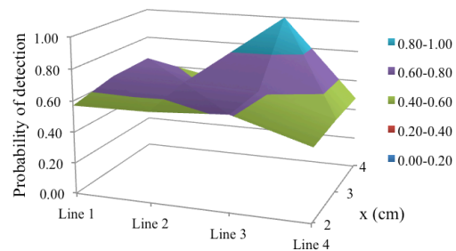
Figure 6: Probability of detection for all positions and a detection threshold r_l = 0.3 cm
