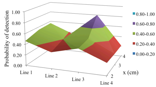
Figure 5: Probability of detection for all positions and a detection threshold r_l = 0.1 cm
