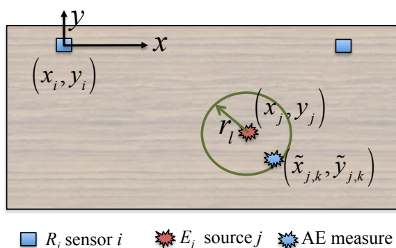
Figure 3: Problem parameterization
