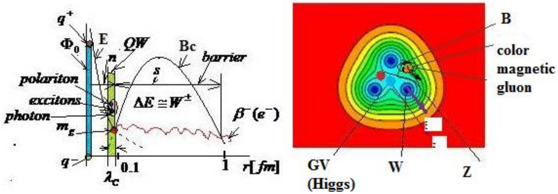
Figure 1.a. The mass generation by dual Meissner effect, the \beta decay for a free neutron and, n -normal vacuum, s -superconductor, QW -quantum well.
