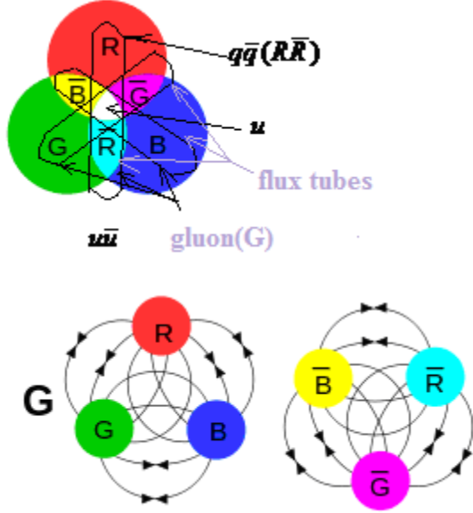
Fig.1.b. Fields due to color charges as in sea quarks ( q\bar{q}(R\bar{R}) ) of valence quarks ( u ), ( \mathbf{G} is the gluon field strength tensor). These are "colorless" combinations. Top: Color charge has "ternary neutral states" as well as binary neutrality (analogous to electric charge).
