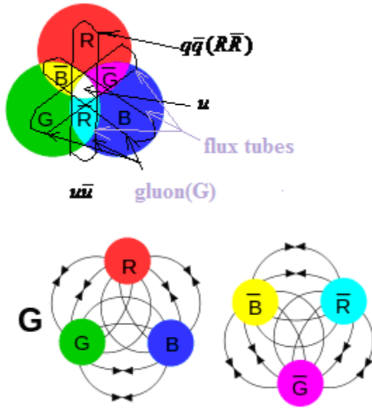
Fig.1.b. Fields due to color charges as in sea quarks ( q\bar{q}(R\bar{R}) ) of valence quarks ( u ), ( G is the gluon field strength tensor). These are "colorless" combinations. Top: Color charge has "ternary neutral states" as well as binary neutrality (analogous to electric charge).
