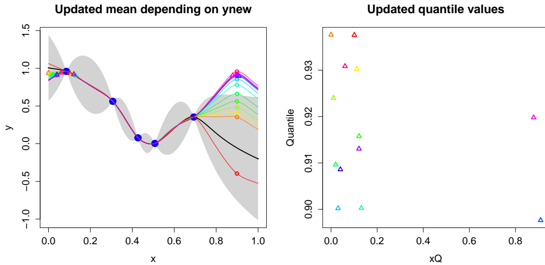
FIGURE 2. Illustration of the J^{\text{Var}} criterion. Left: GP model (black bold line and grey area) and updated GP mean (other lines) depending on the value of g_{new} (circles) for \mathbf{x}_{n+1} = 0.9 . The corresponding 90% percentiles q_{n+1} are shown with the triangles. Right: percentile values only, indexed by the corresponding percentile points.
