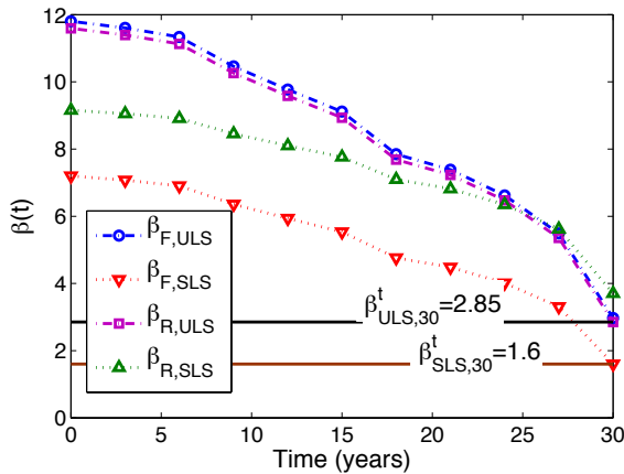
Figure 4: Time-dependent reliability index of TD-RBDO solution for flexible (F) and rigid (R) joints.
