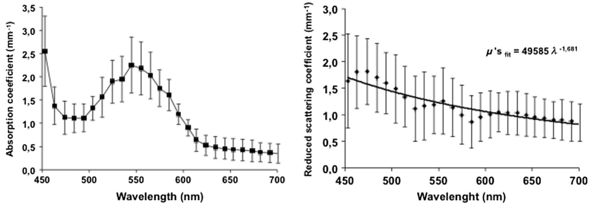
Fig. 2 Optical absorption and reduced scattering coefficients for fresh kidney tissues (3 animals, 6 slices, 8 independent measurement points). Error bars represent one standard deviation.
