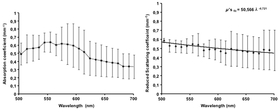
Fig. 6 Optical absorption and reduced scattering coefficients for muscle tissues after cryogenic processing (3 animals, 6 slices, 6 independent measurement points). Error bars represent one standard deviation.
