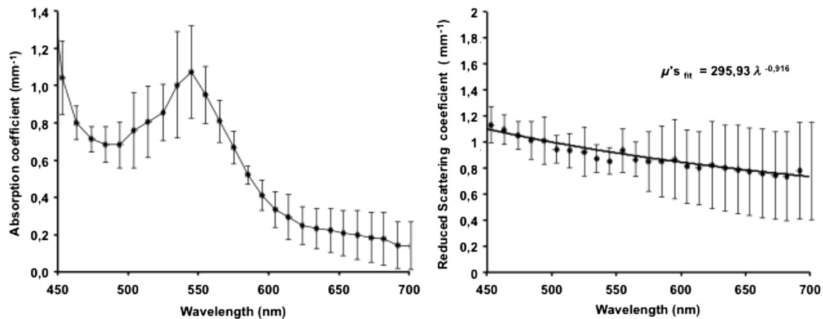
Fig. 5 Optical absorption and reduced scattering coefficients for the liver tissues after cryogenic processing (3 animals, 6 slices, 6 independent measurement points). Error bars represent one standard deviation.
