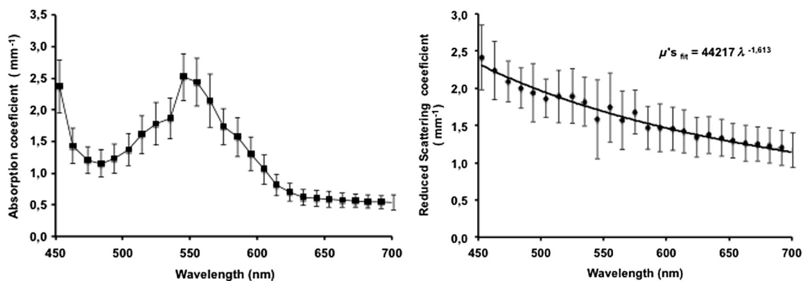
Fig. 1 Optical absorption and reduced scattering coefficients for fresh heart tissues (3 animals, 6 slices, 12 independent measurement points). Error bars represent one standard deviation.
