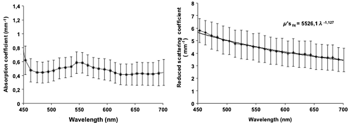
Fig. 3 Optical absorption and reduced scattering coefficients for fresh brain tissues (4 animals, 6 slices, 10 independent measurement points). Error bars represent one standard deviation.
