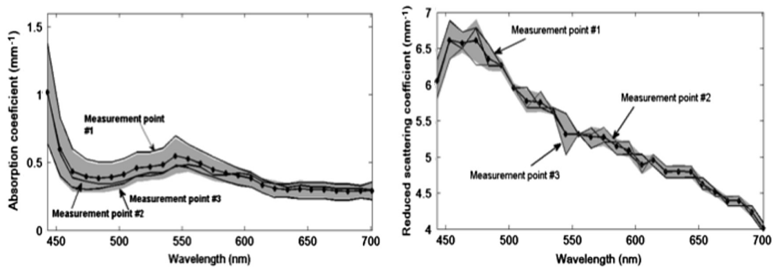
Fig. 7 Intraindividual variability of optical fresh brain optical properties. Intraindividual variability was evaluated from three independent measurements for a single animal at different locations within the gray matter (striata). Thick black line and diamonds are the mean of measurements. Black lines correspond to optical properties derived from single measurements. Shaded gray area corresponds to one standard variation of measurements.
