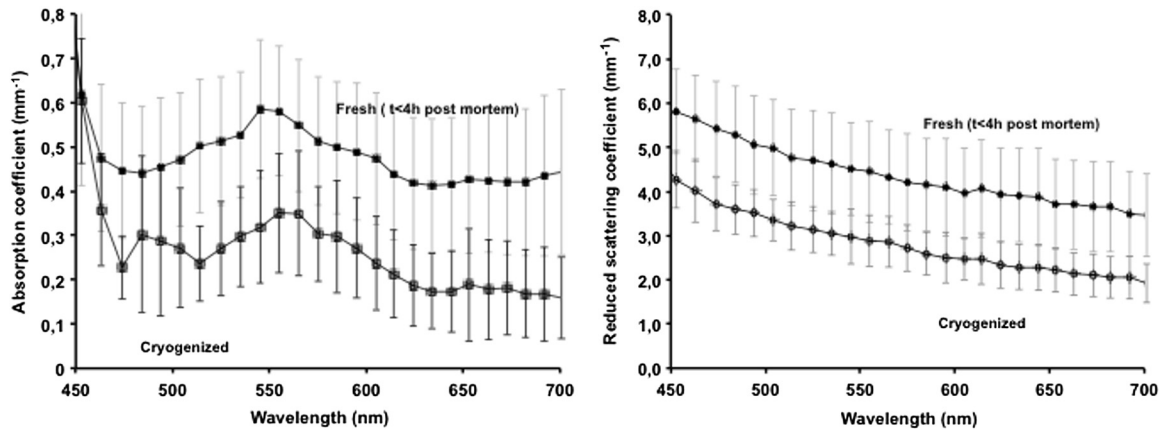
Fig. 4 Influence of cryogenic processing on optical properties of brain tissues (fresh tissues: 4 animals, 6 slices, 10 independent measurement points; frozen tissues, 1 animal, 1 slice, 2 independent measurement points).
