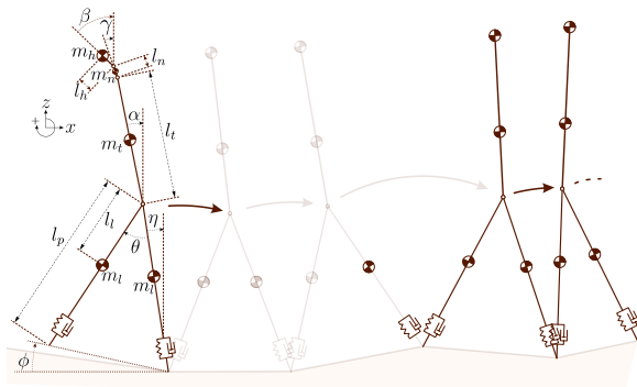
Figure 11. Two control schemes. Model A is subject to the constraints \alpha = \beta = \gamma (rigid neck). Model B has stabilized neck joints.
