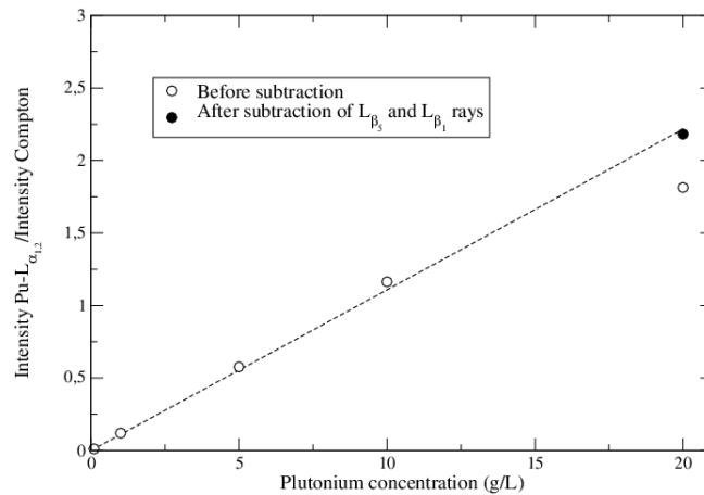
Figure 13: Ratio I_{\text{Pu-L}_{\alpha_{1,2}}}/I_{\text{Compton}} as a function of the plutonium concentration after the subtraction of the Pu-L _{\beta_5} and the Pu-L _{\beta_1} peaks.
