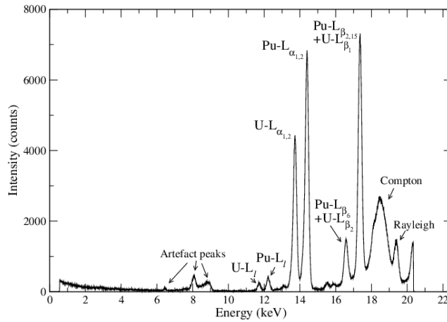
Figure 4: Active spectrum of a plutonium sample at 19.98 \text{ g}\cdot\text{L}^{-1} in 10% \text{HNO}_3 , analysed during 300 seconds.
