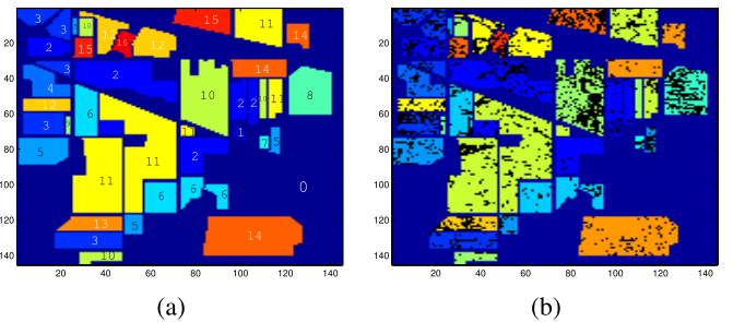
Fig. 13. Detection of nonlinearly mixed pixels in Indian Pines hyperspectral image. Black pixels were detected as nonlinearly mixed ones by the proposed detector. (a) Indian Pines ground truth. (b) Indian Pines detection map.
