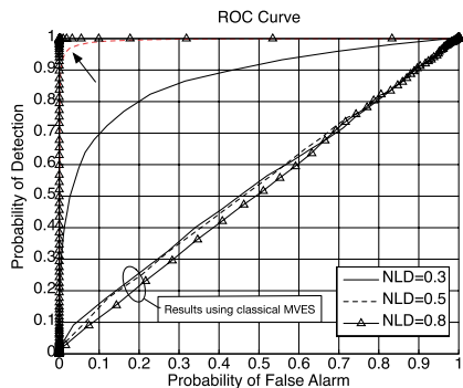
Fig. 5. ROCs for different degrees of nonlinearity \eta_d and 50% of nonlinearly mixed pixels in the image. Endmember extraction using Algorithm 1
