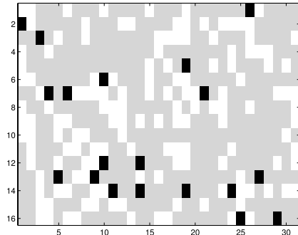
Fig. 11. Detection map and true nonlinear map. Linearly mixed pixels in gray, nonlinearly mixed pixels in white, and misclassified pixels in black.
