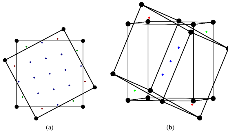
Fig. 4. Visualization of qw \in q\mathcal{C}(\mathbf{0})\bar{q} \cap |q|^2\mathcal{C}(\mathbf{0}) – in blue, qw \in q\mathcal{C}(\mathbf{0})\bar{q} \setminus |q|^2\mathcal{C}(\mathbf{0}) – in red, and |q|^2\mathcal{C}(\mathbf{0}) \setminus q\mathcal{C}(\mathbf{0})\bar{q} – in green, for (a) q = 4 + k and (b) q = 2 - 3i - 2j - 5k , each of which induces a non-bijective digitized rational rotations.
