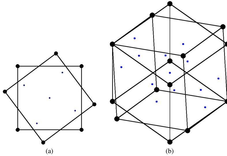
Fig. 3. Visualization of qw \in q\mathcal{C}(\mathbf{0})\bar{q} \cup |q|^2\mathcal{C}(\mathbf{0}) together with q\mathcal{C}(\mathbf{0})\bar{q} and |q|^2\mathcal{C}(\mathbf{0}) , for (a) q = 3 + k and (b) q = 3 + 4i + k , each of which induce bijective digitized rational rotation. Points qw are depicted as blue spheres.
