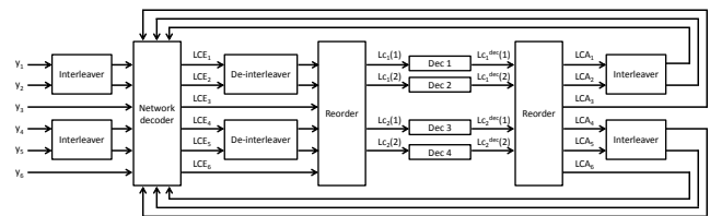
Fig. 2. Structure of the joint network-channel decoder at the destination.
