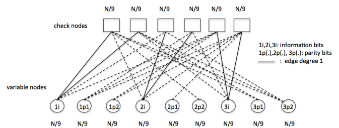
Fig. 3. Tanner graph of a root LDPC decoder with R = 1/3 .
