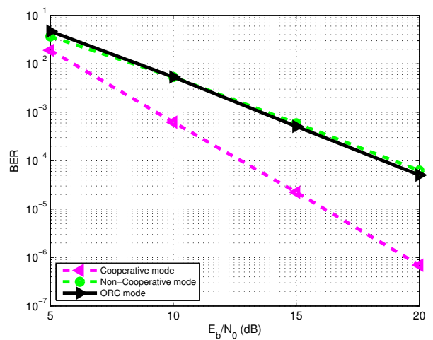
Fig. 4. BER comparison. The two sources are equidistant from the relay and the destination with d_{S_1R} = d_{S_2R} = d_{RD} \approx 0.5 , d_{S_1D} = d_{S_2D} \approx 1 and \alpha = 2 .
