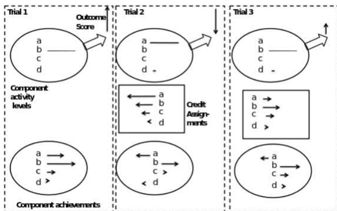
Fig. 3. Correlation algorithm for computing component achievements.
