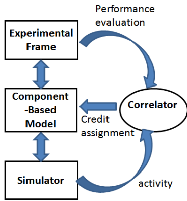
Fig. 2. Basic modeling and simulation entities in activity-based credit assignment.
