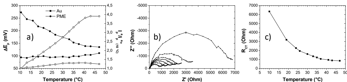
Fig.3 (a) \Delta E_p (filled symbols) and r (open symbols) vs. temperature (50 mV.s -1 ) on bare Au (squares) and on PME (circles) electrodes, (b) EIS: full circle corresponds to 14 Hz. From largest to smallest semi-circle: 10; 19; 24; 26; 30; 35 and 47 °C and (c) R_{CT} vs. temperature for the PME.
