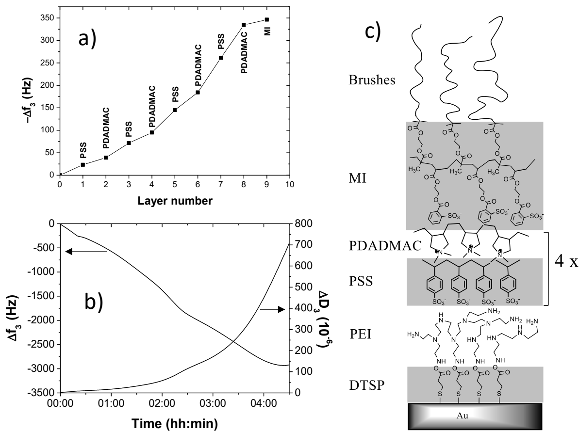
Fig.1 Resonance frequency and dissipation shift monitored by E-QCM-D upon (a) LBL assembly by successive deposition of PSS and PDADMAC and finally of the macroinitiator MI, and (b) polymerization from the pre-modified electrode surface. (c) Proposed structure of the smart PME (scheme)
