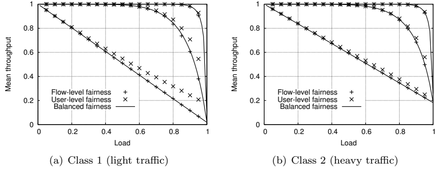
Figure 6: Impact of fairness on throughput performance under the multi-source model for m = 1, 10, 100 (from bottom to top) and n_1 = n_2 = 5m .
