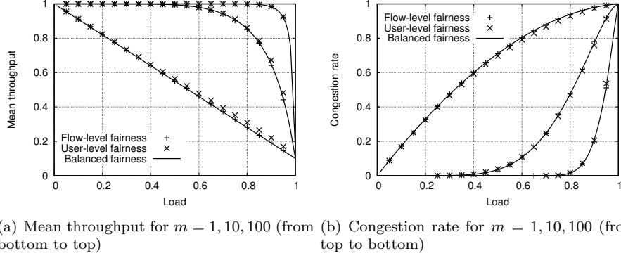
Figure 5: Impact of fairness on performance under the multi-source model for n = 10m .
