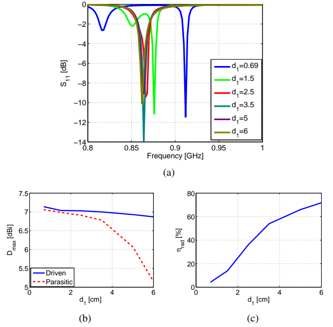
Fig. 3. Parasitic two-element array parameters as a function of the inter-element distance. (a) simulated input reflection coefficient magnitude in dB, (b) total directivity, and (c) radiation efficiency.
