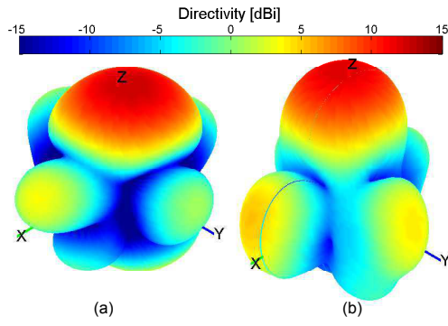
Fig. 7. Planar array 3D total directivity radiation pattern for d=26\text{cm} . (a) Simulated and (b) measured.
