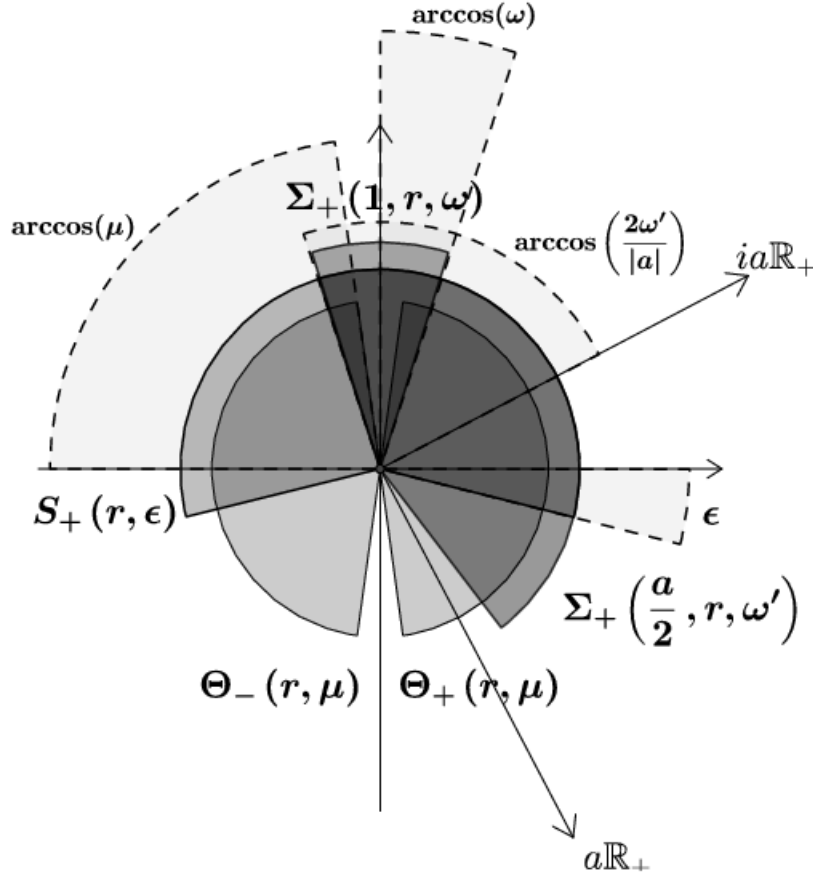
Figure 1: representation of domains \Sigma_+(1, r, \omega) , \Sigma_+(\frac{a}{2}, r, \omega') , \Theta_+(r, \mu) , \Theta_-(r, \mu) , S_+(r, \epsilon) , without the appropriate radius.
