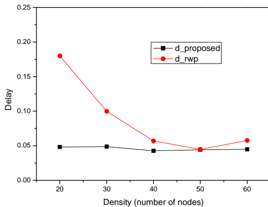
Fig. 7. Average end-to-end delay varying node density
