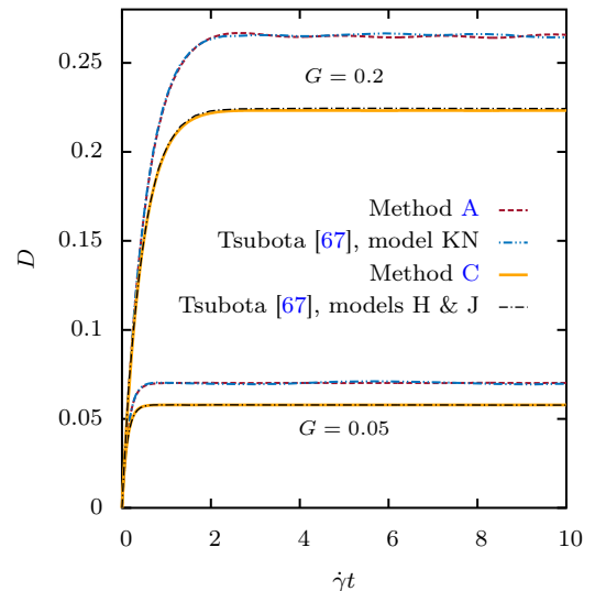
Figure 17: Comparison of the deformation parameter for \hat{\kappa}_B = 2/15 (once for G = 0.05 and once for G = 0.2 ) for Methods A and C with Tsubota 2014 [67]. 5120 triangles. Method A is virtually identical to model KN from [67], Method C is essentially alike to model H. Note that Tsubota uses BIM, 4604 flat triangles and the same physical conditions.
