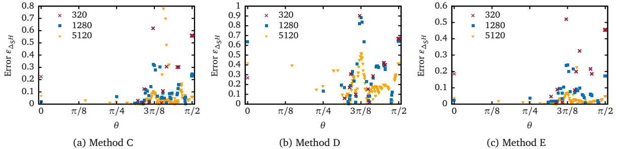
Figure S7: The numerical error \varepsilon_{\Delta_S H} upon evaluating the Laplace-Beltrami operator on the mean curvature. MT1 meshes. The graphs for \Delta_S H can be found in figure 6 in the main text.
