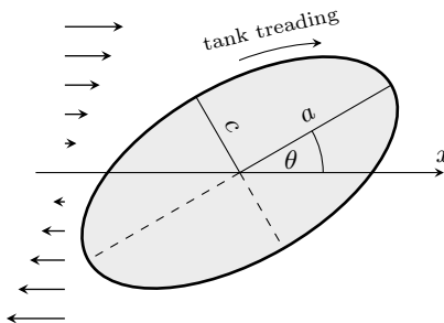
Figure 11: 2D illustration of the linear shear system. The actual simulation is three-dimensional. The spherical capsule deforms into an ellipsoid-like shape. a is the largest and c the smallest half axis, while \theta is the inclination angle. The membrane rotates around the object’s centroid (the so-called “tank-treading” motion).
