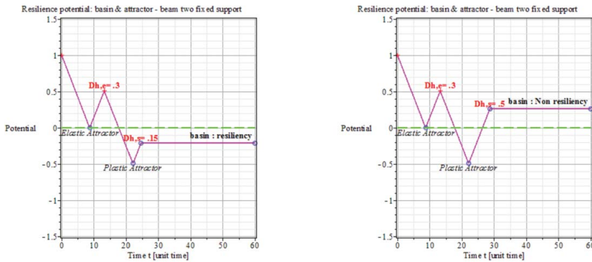
(a)- Resilient tank: D_h^{\text{edge}} = 0.3; D_h^{\text{span}} = 0.15 (b)- Non-resilient tank: D_h^{\text{edge}} = 0.3; D_h^{\text{span}} = 0.5
