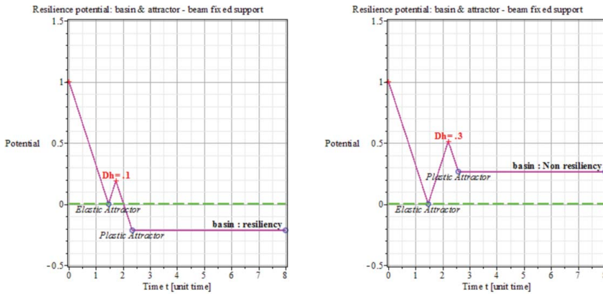
(a)- Resilient tank: D_h = D_h^{\text{edge}} = 0.1 (b)- Non-resilient tank: D_h = D_h^{\text{edge}} = 0.3
