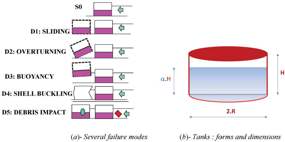
Figure 8. Cylindrical metal tanks for storing oil in industrial plants: (a) failure modes of tanks; (b) various dimensions: 5 sizes \{T_1: H = 8 \text{ m}, R = 5.57 \text{ m}\}; \{T_2: H = 10 \text{ m}, R = 14 \text{ m}\}; \{T_3: H = 19 \text{ m}, R = 10 \text{ m}\}; \{T_4: H = 30 \text{ m}, R = 20 \text{ m}\}; \text{and} \{T_5: H = 30 \text{ m}, R = 40 \text{ m}\}.
