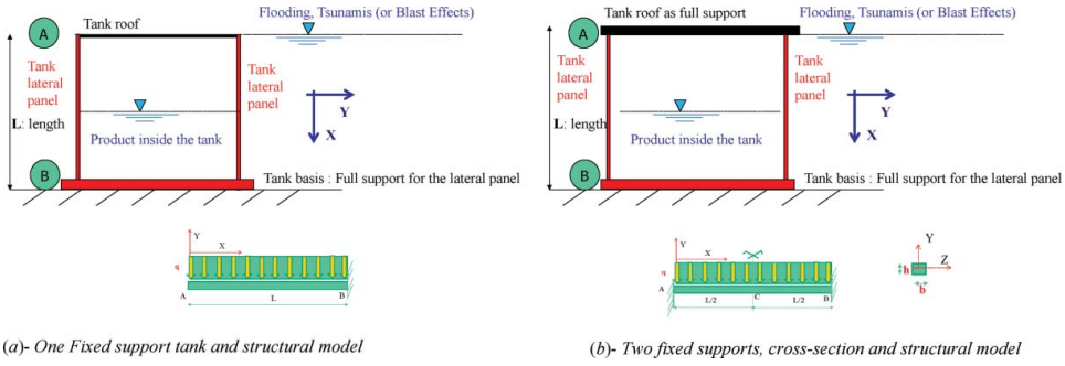
Figure 2. Metallic tanks and equivalent structural beam models under uniform lateral pressure. (a) One fixed support tank and structural model and (b) two fixed supports, cross-section and structural model.
