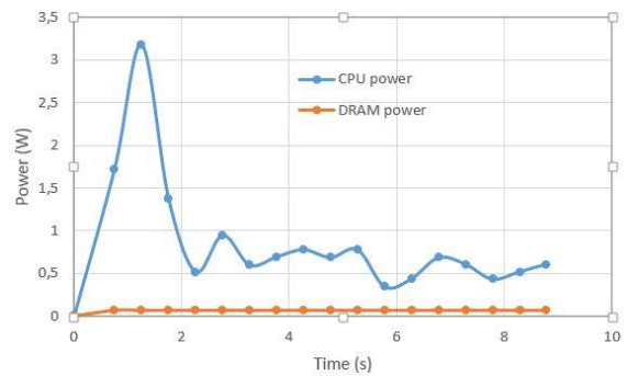
Figure 4.b: Subexpression optimized.
