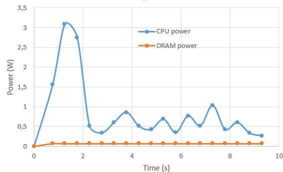
Figure 4.a: Subexpression unoptimized.
