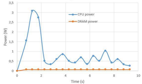
Figure 4.a: Subexpression unoptimized.
