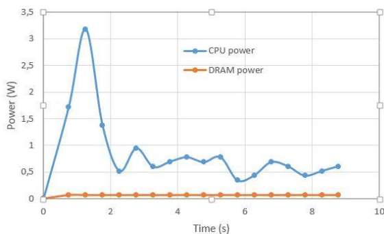
Figure 4.b: Subexpression optimized.
