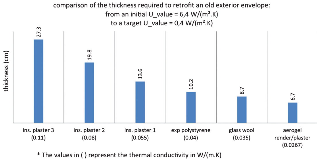
Fig. 1. Comparison of the thickness required to retrofit an old exterior envelope from an initial U -value of 6.4 W/(m 2 K) to a target U -value of 0.4 W/(m 2 K) with different insulating materials (Ibrahim et al., 2015a).
