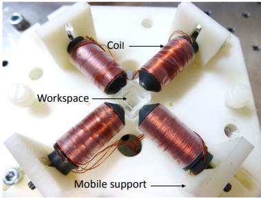
Fig. 1. Non contact magnetic actuation device: four coils create a magnetic force to control the position of the robot. They are placed on a mobile support to adapt the gap between the coils to the size of the workspace.
