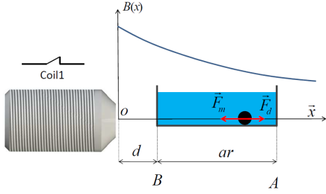
Fig. 3. Configuration of the system when the coil 1 is actuated : the workspace is located at a distance d from coil 1 and the microrobot moves under the action of the magnetic field B to cover the distance w = ar from A to B . F_m and F_d are the magnetic and the drag force respectively.
