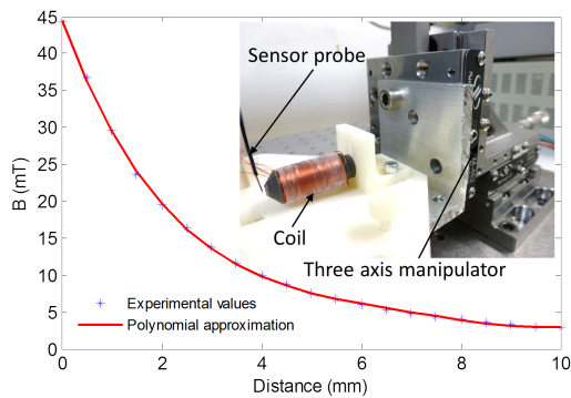
Fig. 4. Experimental setup used for the magnetic field measurement along the coil axis: an Hall sensor measures the magnetic field. A 3 axis manipulator controls the distance between the coil and the magnetic probe.
