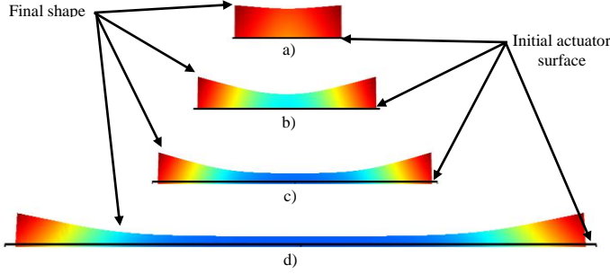
Fig. 5. Diagonal section view of free side behaviour for different actuator widths at an applied voltage of 400V: a)250x250µm²; b)300x300µm²; c)400x400µm²; d)800x800µm². PMN-PT thickness is 200µm.
