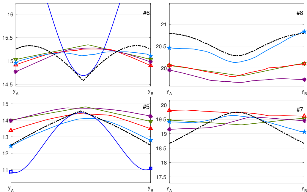
Above: The eigenvalues #5-6 switch (left). The eigenvalues #7-8 come close (right). The Smolyak interpolant for #7-8 is outside the range shown.
