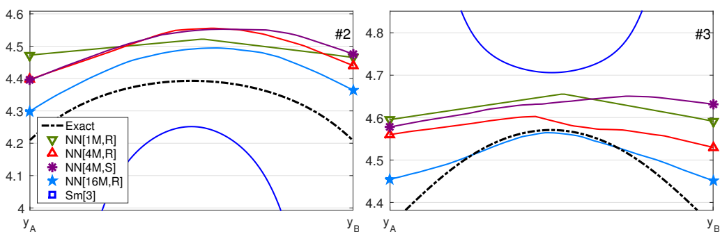
Above: The eigenvalues #2-3 are slightly distinct (due to discretization asymmetry).
