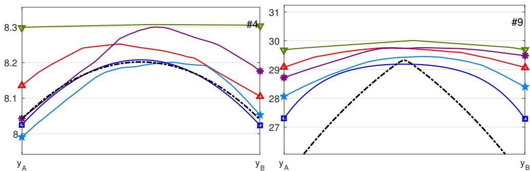
Above: The simple eigenvalues #4 and #9. Eigenvalue #9 comes close to #10 midway.
