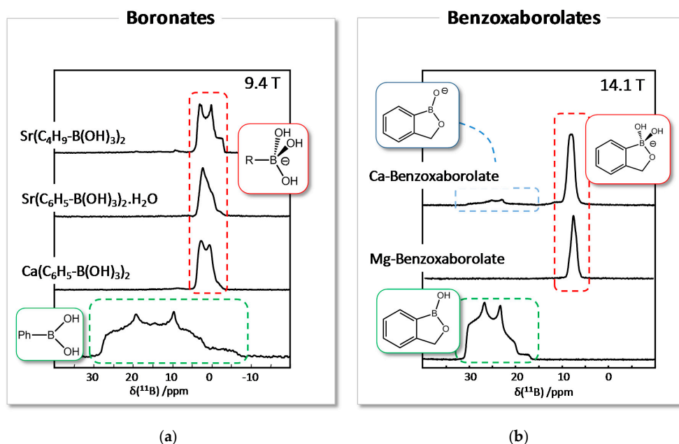
Figure 9. ^{11}\text{B} solid state NMR spectra of alkaline-earth metal boronates (a) and benzoxaborolates (b), as well as for the corresponding boronic acid and benzoxaborole. The spectra shown here were recorded under MAS at two different magnetic fields (9.4 T for boronic acids, vs. 14.1 T for benzoxaboroles), and present second order quadrupolar lineshapes. Adapted with permission from [27] (copyright American Chemical Society, 2015).
