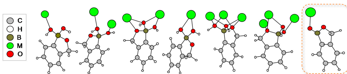
Figure 8. Coordination modes of the simplest benzoxaborolate ligand with respect to alkaline earth metals ( M = Mg, Ca ). The deprotonated benzoxaborolate found in the Ca structure is outlined in dashed orange. Adapted with permission from [27] (copyright American Chemical Society, 2015).
