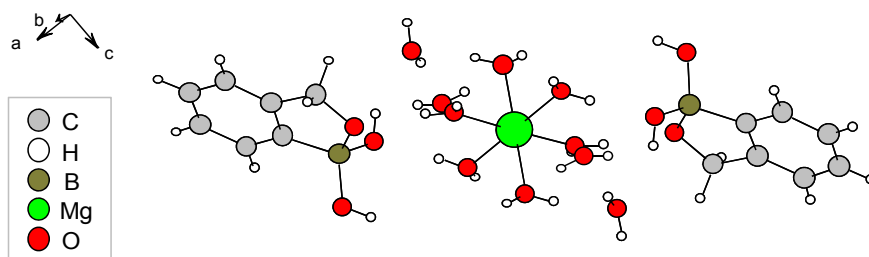
Figure 7. Coordination environment of Mg^{2+} in the Mg-benzoxaborolate decahydrate phase, showing that the metal cation is linked to 6 water molecules, while the benzoxaborolate anions balance the charge [27].
