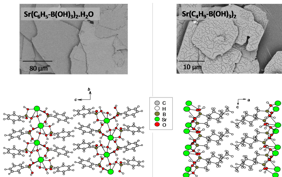
Figure 4. SEM images and crystal structures of \text{Sr}(\text{C}_6\text{H}_5-\text{B}(\text{OH})_3)_2 \cdot \text{H}_2\text{O} (left) and \text{Sr}(\text{C}_4\text{H}_9-\text{B}(\text{OH})_3)_2 (right). Adapted with permission from [22] (copyright American Chemical Society, 2011), [24] (copyright Wiley-VCH Verlag 2013) and [25] (copyright Actualité Chimique, 2014).
