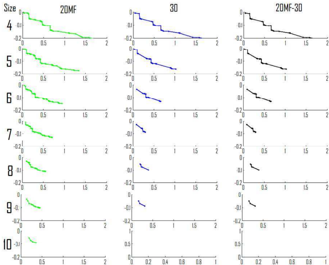
Figure 8. filter Pareto fronts in (-D, R) space from size 4 to 10 for wineWhite (11 features) database during 2OMF , 30 and 2OMF-30
