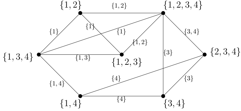
Figure 1: Example of a union vertex-distinguishing coloring
