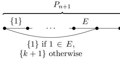
Figure 8: The construction of C_n from P_{n+1} .
