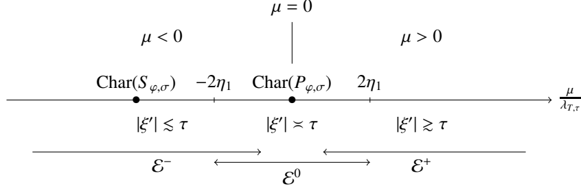
Figure 2: Representation of the three microlocal regions.
