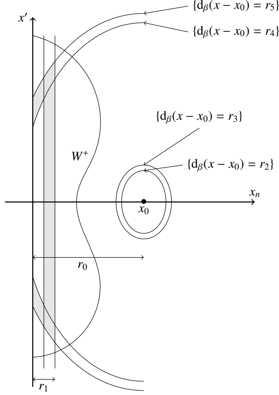
Figure 4: Geometry of the cut-off functions near (0, 0) . The grey zone corresponds to the region where \chi_0\chi_1 varies.
