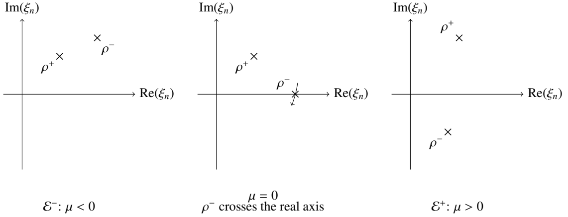
Figure 1: Position of the roots of p_{\varphi,\sigma} as \mu varies.
