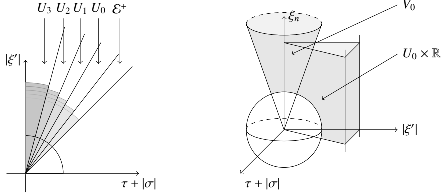
Figure 3: Representation of the different conic neighborhoods.
