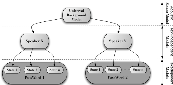
Figure 1: General view of the EBD model architecture.
