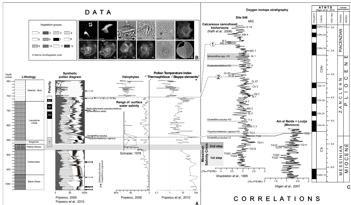
Fig. 1. Chronostratigraphic and environmental data on the lower part of Hole 380A (1019.85–645 mbsf) and proposed correlations.
