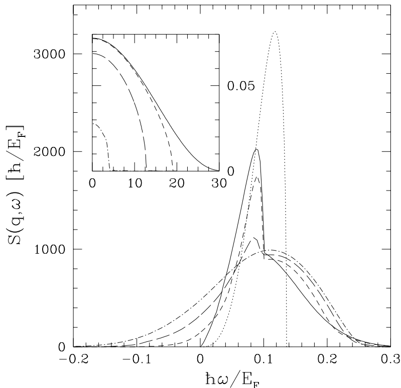
FIG. 2: Dynamic structure factor of a confined superfluid Fermi gas for \hbar q = 4.15 p_{ho} at different temperatures: T = 0 (solid line), k_B T = 0.014 E_F (short-dashed line), k_B T = 0.028 E_F (long-dashed line) and k_B T = 0.042 E_F (dot-dashed line). The critical temperature for the BCS transition is k_B T = 0.047 E_F . The analytic expression for the broadening of the Bogoliubov-Anderson phonon in the low q and zero temperature limit, Eq. (27), is given in dotted line. The inset shows the gap function in units of E_F as a function of the radial coordinate r/a_{ho} , as obtained from the local-density approximation. The different line-styles correspond to the different temperatures of the main figure. p_{ho} = \sqrt{\hbar m \Omega} , a_{ho} = \sqrt{\hbar/m\Omega} and E_F is the Fermi energy of a harmonically trapped non-interacting Fermi gas with the same number of particles, E_F = (3N)^{1/3} \hbar \Omega . The parameters used are N = 8 \times 10^7 , \Omega = 2\pi \times 27.2 \text{ s}^{-1} and a_{\uparrow\downarrow} = -2160 a_0 where a_0 is the Bohr radius. These parameters correspond to the weakly-interacting regime with 2k_F |a_{\uparrow\downarrow}|/\pi \simeq 0.4 and to the collisionless regime \omega \tau \gg 1 , where \omega = \hbar c_B q , \tau^{-1} \simeq \pi^3 n a_{\uparrow\downarrow}^2 v_F (T/T_F)^2 , v_F is the Fermi velocity and n is the density at the center of the trap.
