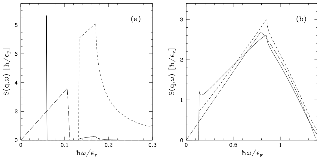
FIG. 1: Dynamic structure factor of a homogeneous superfluid Fermi gas at T = 0 for q = 0.054 k_F (a), and for q = 0.54 k_F (b), as predicted by the RPA (solid line) and by the static Bogoliubov approximation (dashed line). The results for a non-interacting Fermi gas (long-dashed line) are also shown. k_F is the Fermi wavevector and \epsilon_F = \hbar^2 k_F^2/2m is the Fermi energy of the non-interacting Fermi gas at the same density. The parameters chosen are \Delta = 0.065\epsilon_F and k_F a_{\uparrow\downarrow} = -0.04 .
