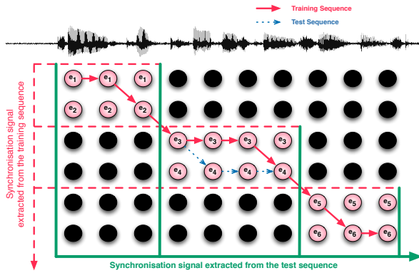
Figure 3: Alignment for client training and test utterances with an external synchronisation.
