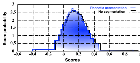
Figure 8: Evolution of the impostors text-dependent scores distributions with or without external synchronisation constraint.
