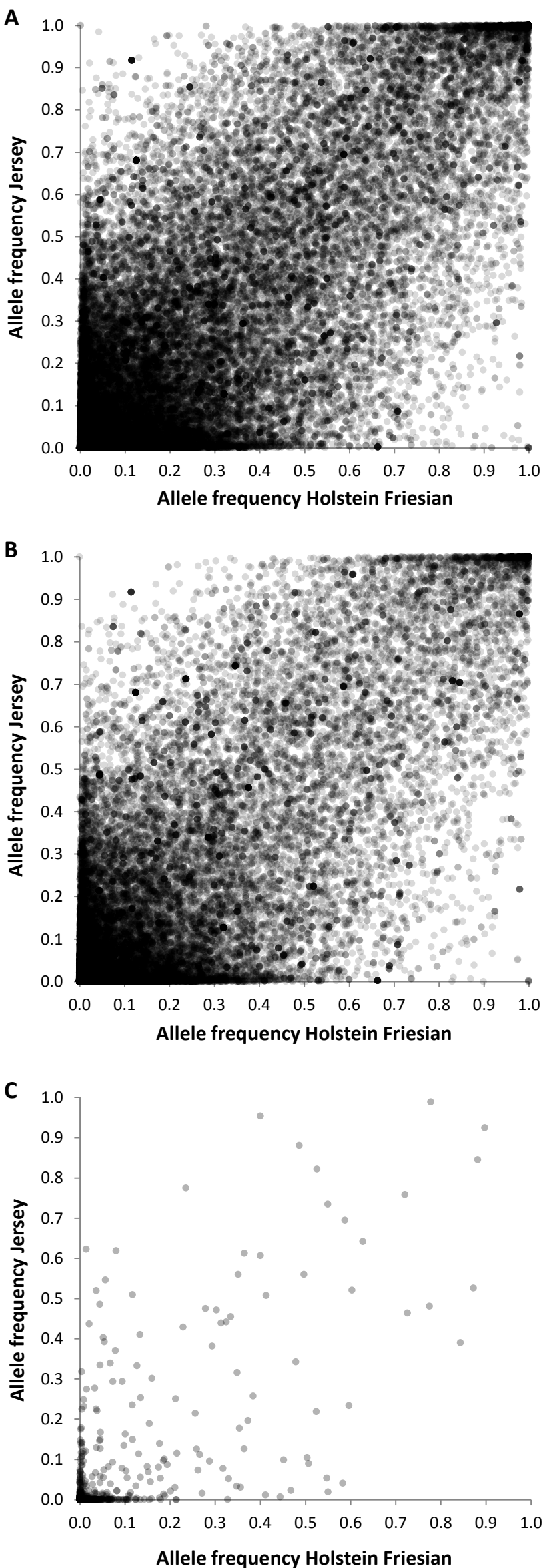
Figure S3 - Allele frequencies of Holstein Friesian versus Jersey animals. Patterns of allele frequencies for Holstein Friesian versus Jersey animals. (A) Variants with on average a moderately low minor allele frequency; (B) Variants with on average a very low minor allele frequency; (C) Variants with on average an extremely low minor allele frequency.
